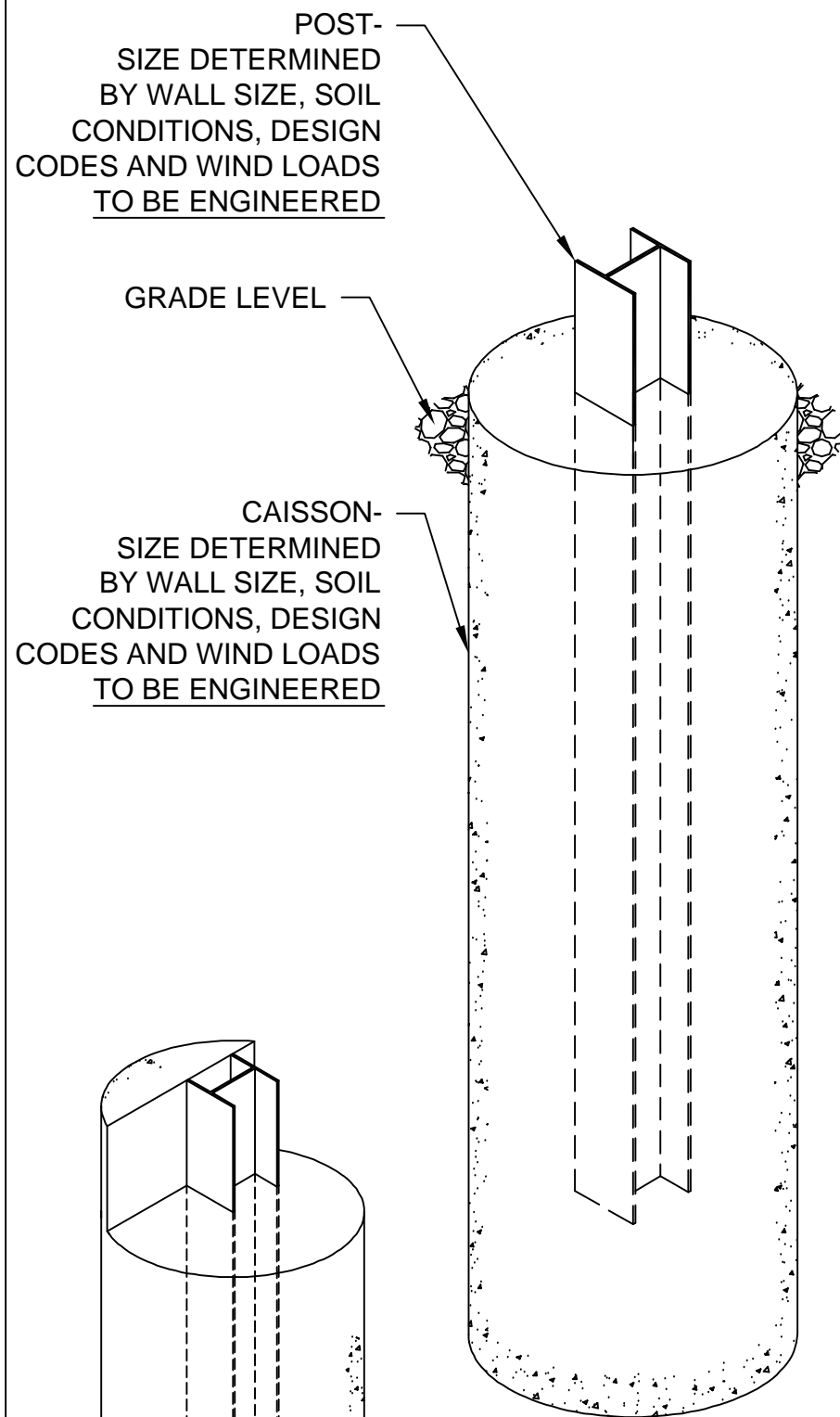
FOUNDATIONS EMBEDDED POST
