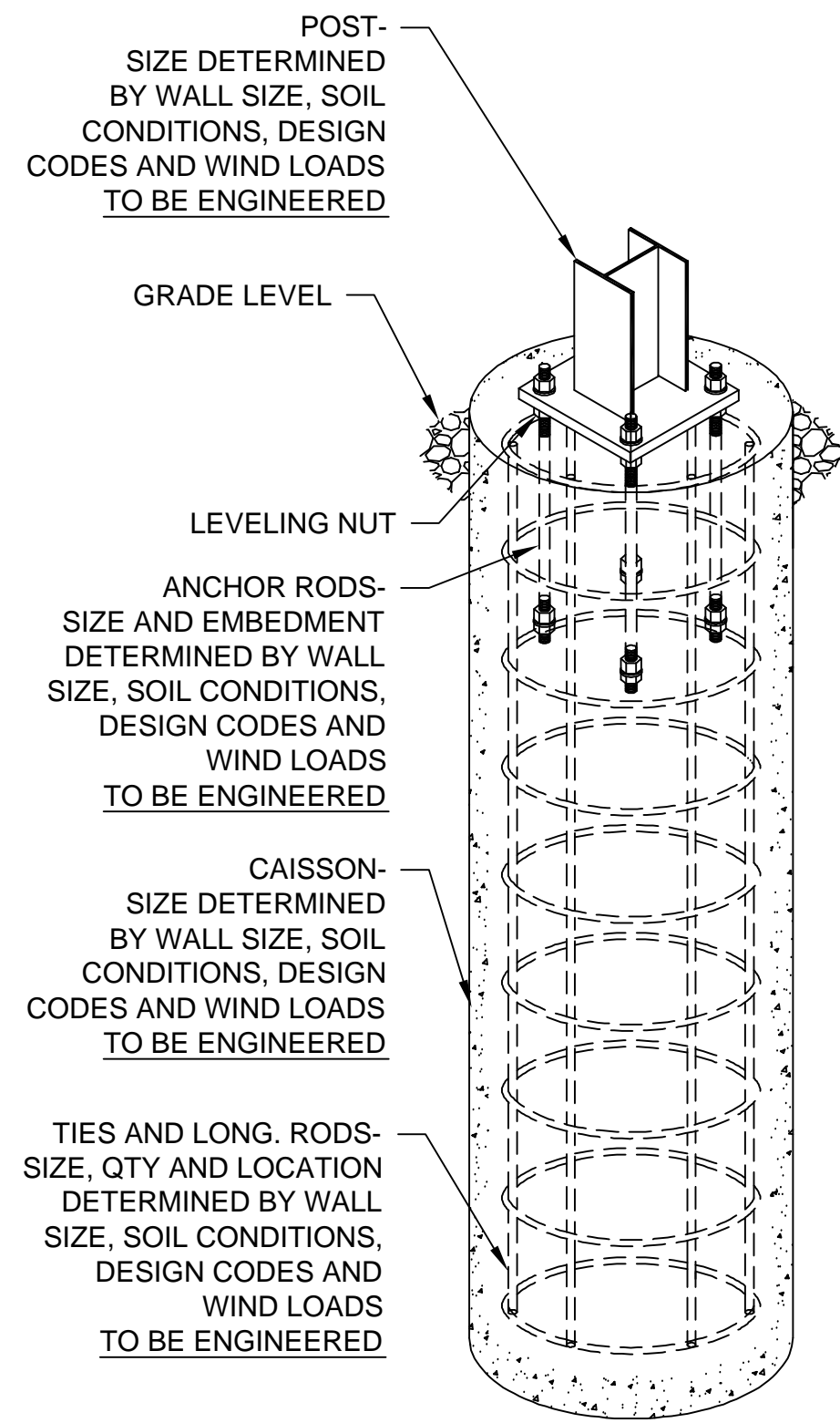
FOUNDATION BASE PLATE POST
