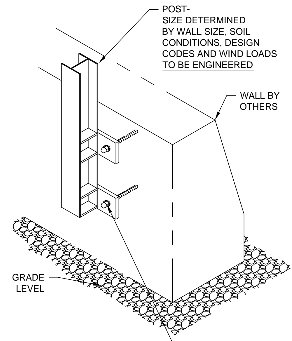
FOUNDATION WALL MOUNTED POST
